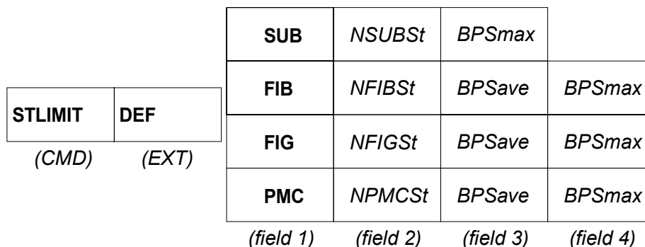
Figure 47: STLIMIT DEF message structure
