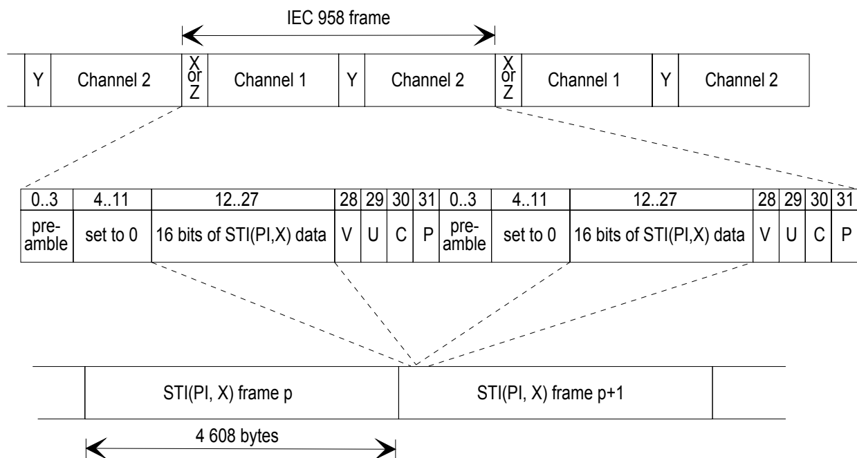
Figure 81: Physical adaptation of STI in the IEC958 frame
