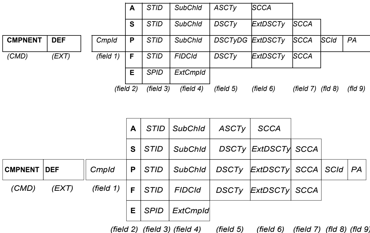
Figure 25: CMPNENT DEF message structure
