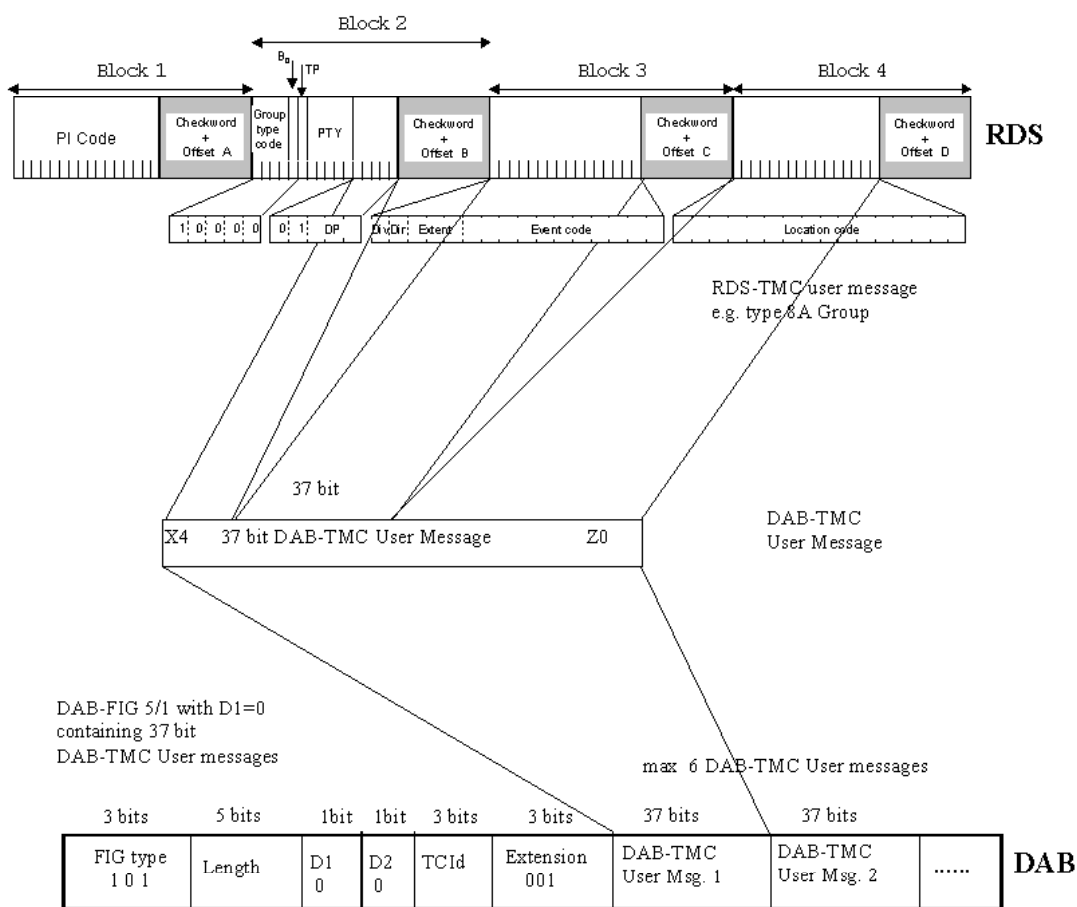
Figure 4: Mapping of 37-bit TMC messages in FIG 5/1 data field (example shown is TMC User Message)
