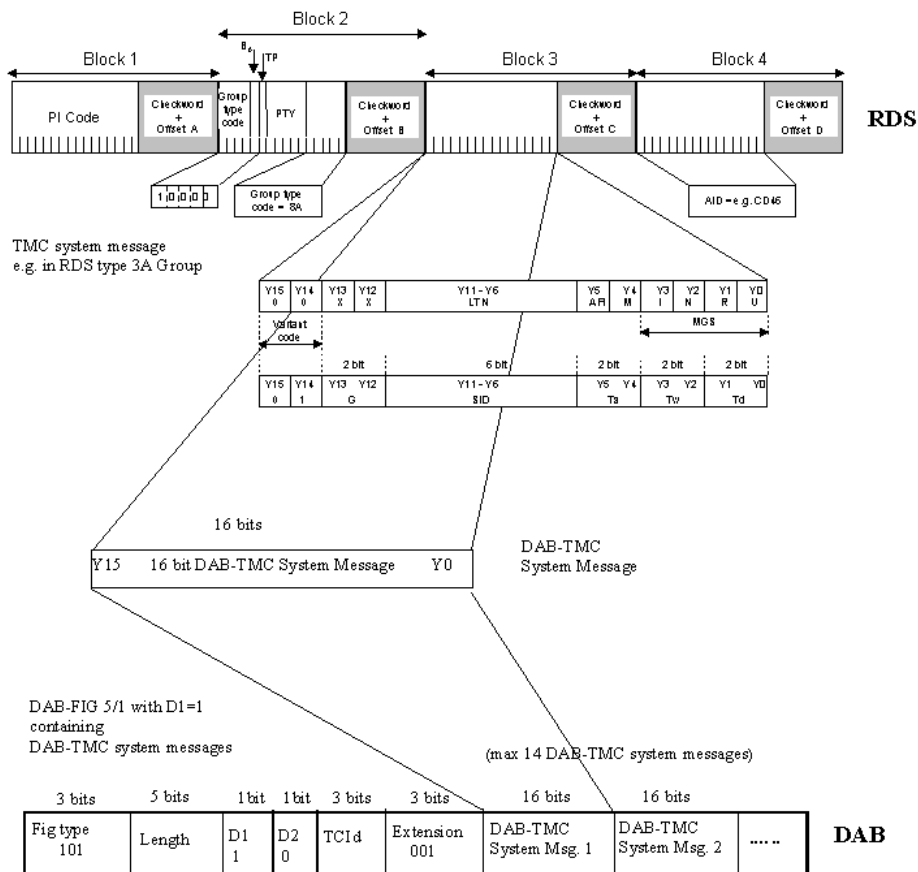
Figure 5: mapping of 16-bit TMC messages in FIG 5/1 (example shown is TMC System Message)
